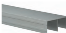
• PPFSA2/3
